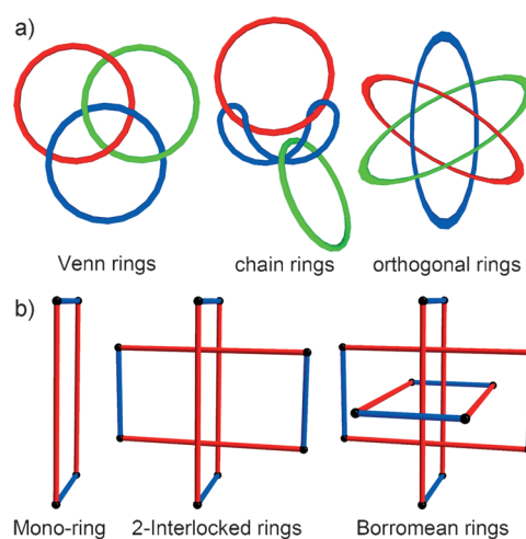
Scheme 1. a) Three representations of the molecular Borromean link. b) The noncatenane n -interlocked rectangles ( n = 2 or 3 ).
